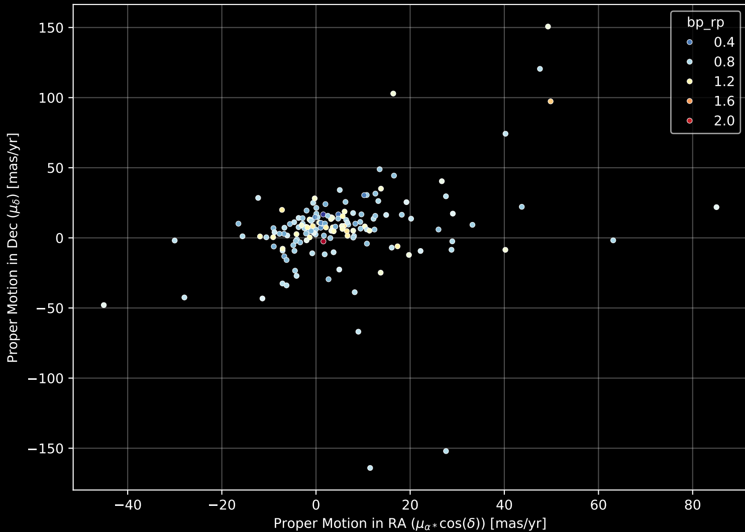
GALAH DR4 Field: [7184] Proper Motion Diagram (n= 151)
