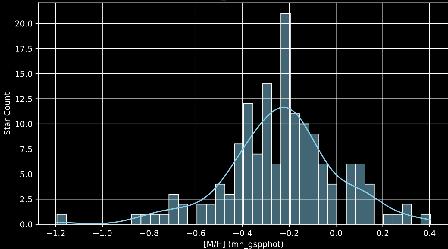
GALAH DR4 Field: [7184] [M/H] (mh_gspphot) (n= 150)
