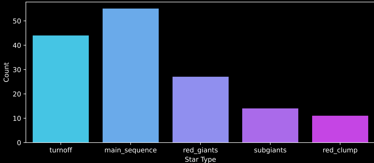
GALAH DR4 Field: [7184] Count plot of Star Type
