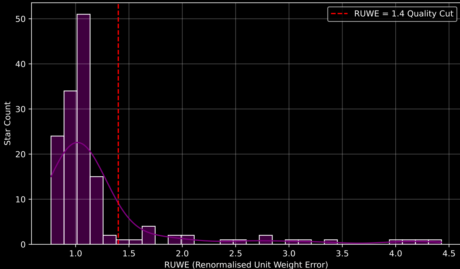
GALAH DR4 Field [7184] RUWE Distribution (n= 147)
