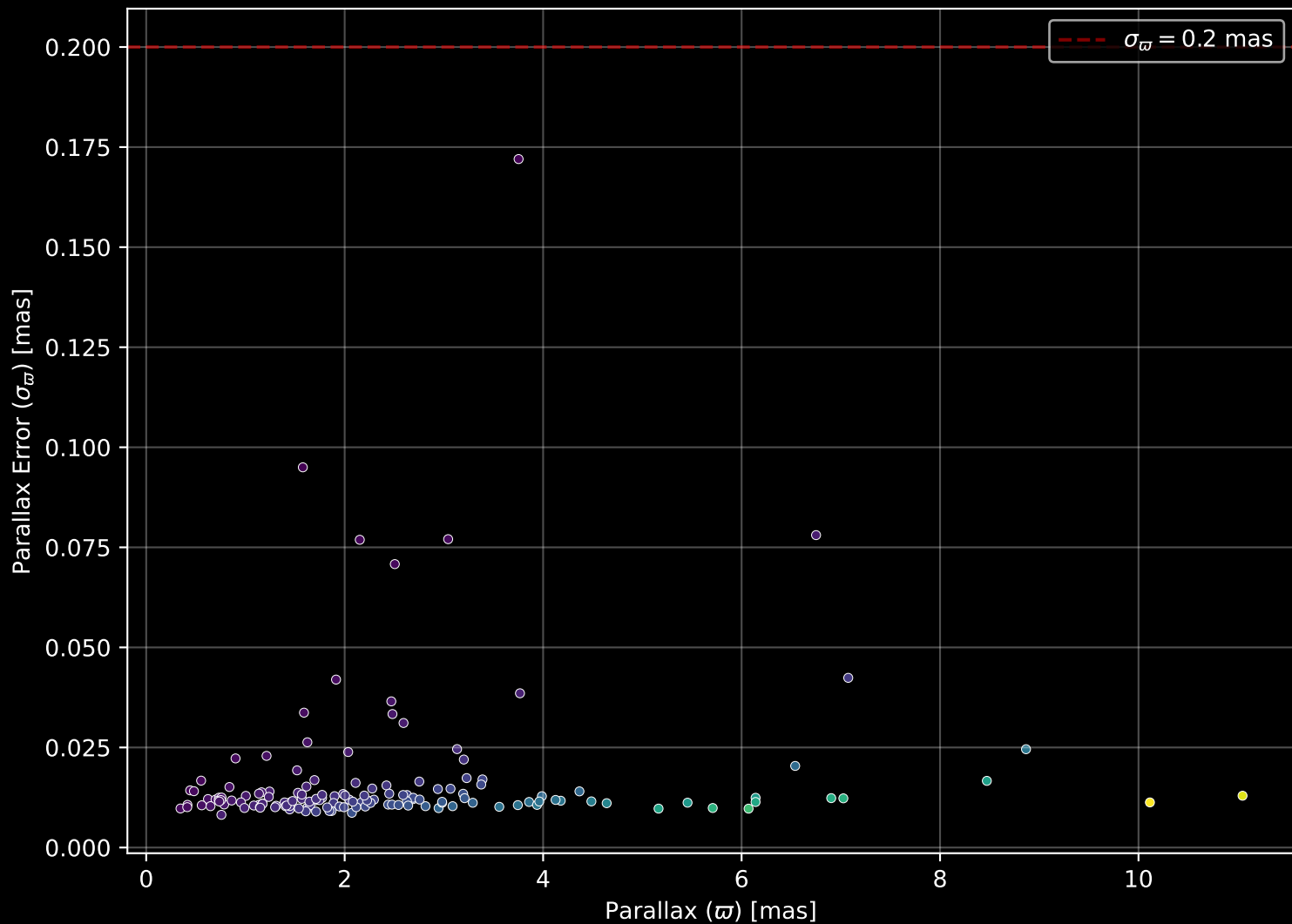
GALAH DR4 Field: [7184] Parallax Quality (n= 151)
